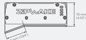
IT300-S CHINE STBD
