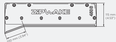
IT450-S CHINE STBD
